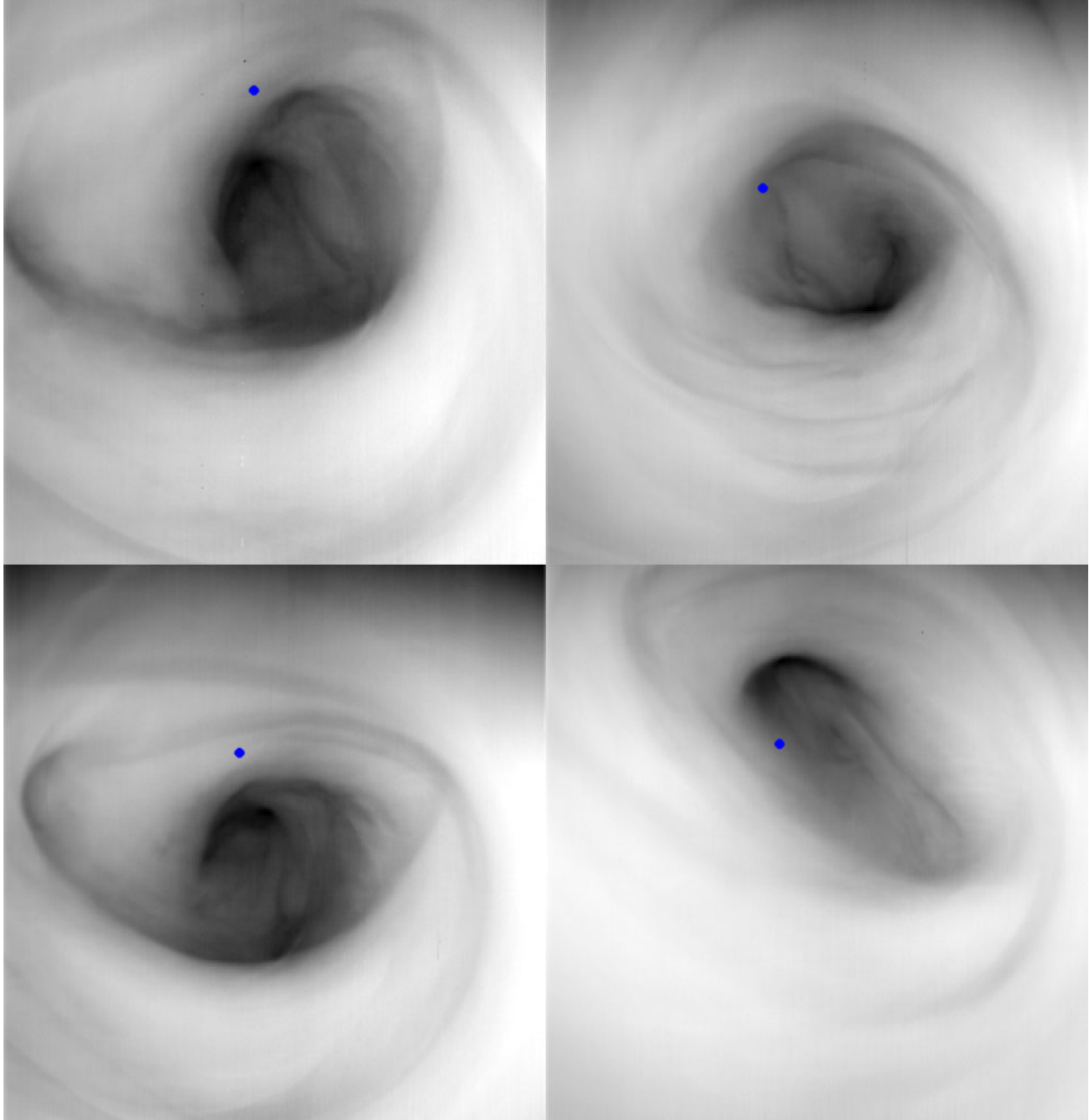
The South Polar Opening of Venus, photos taken by the European Space Agency's robotic Venus Express spacecraft
